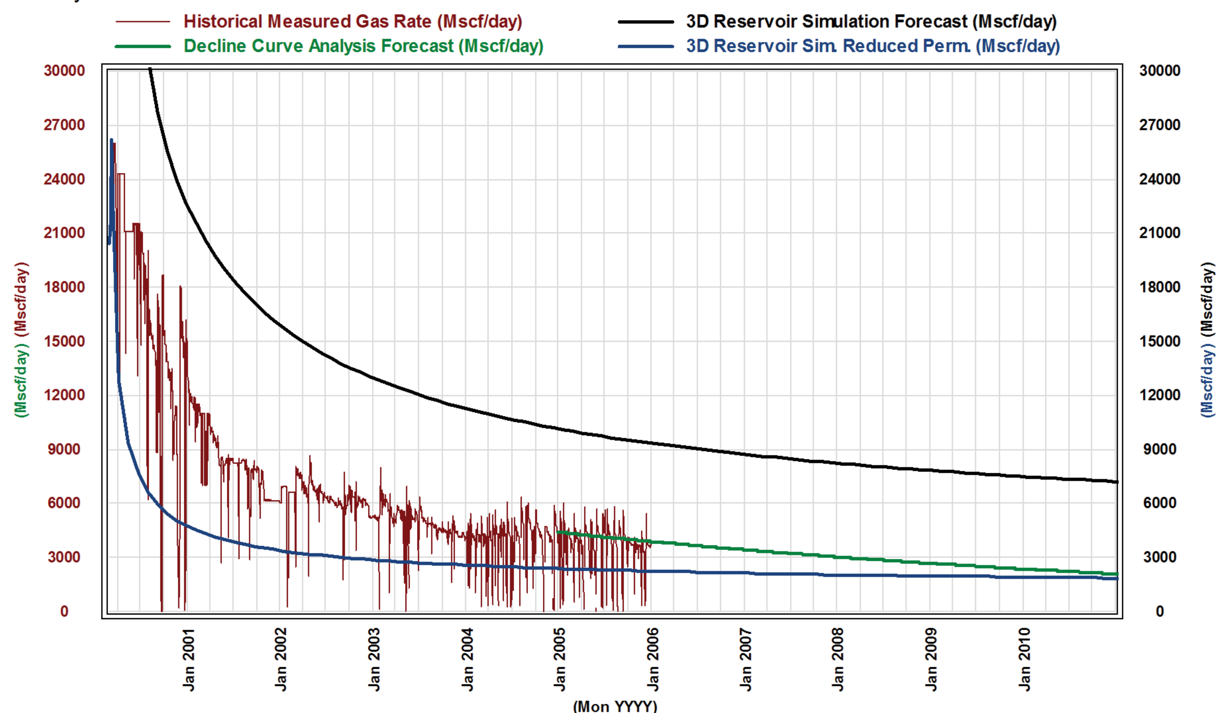
3D Reservoir (Original vs. Reduced Perm.) & Decline Curve
